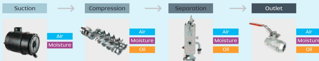
Oil Lubricated Compressor
